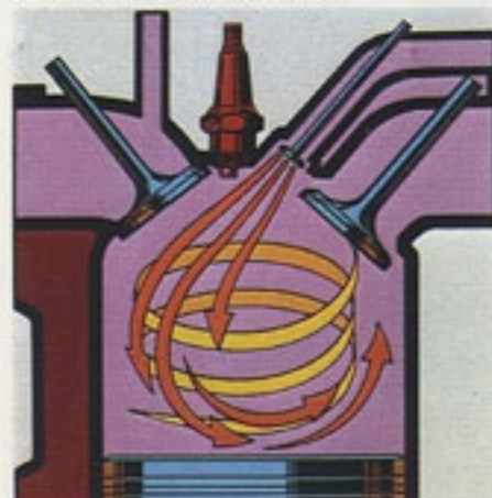
MCA-Jet Engine Piston Chamber
