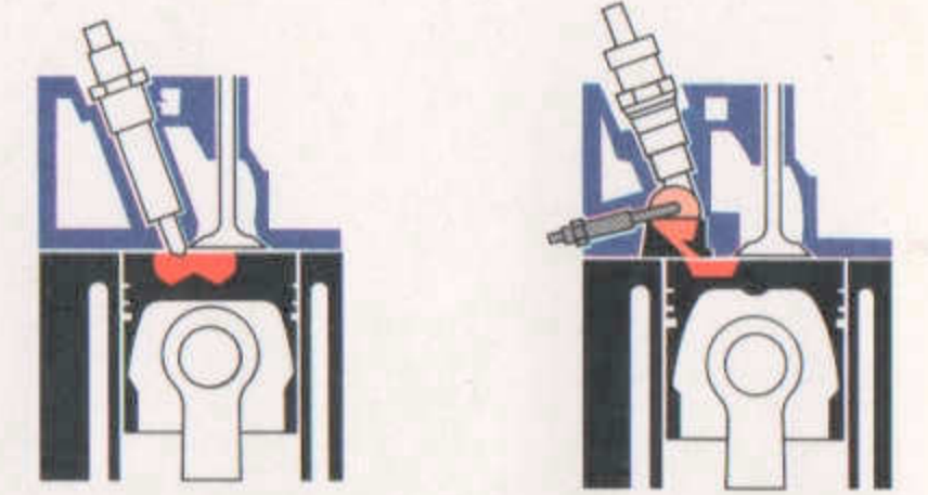
Cummins direct-chamber injection.
